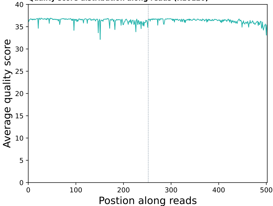
Quality score distribution along reads (R10120)
